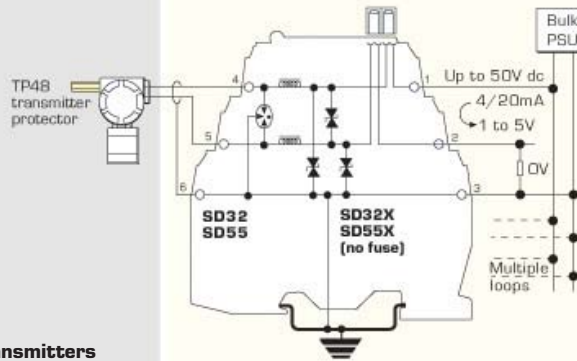
2-wire transmitters
