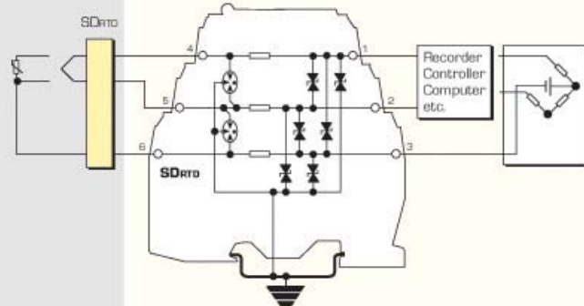
3-wire RTDs
